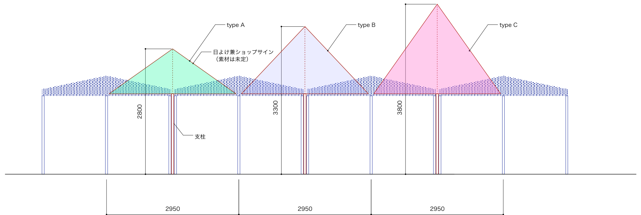
elvation S=1/50
